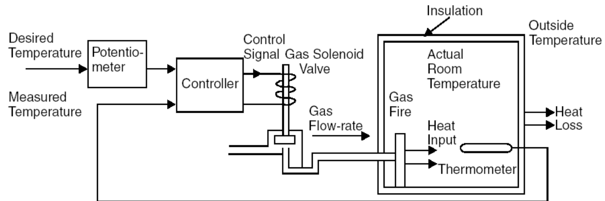
Fig. 1.6 Room temperature control system.
