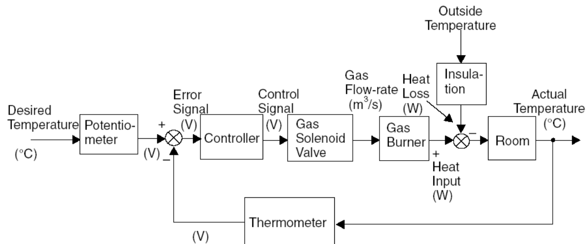
Fig. 1.7 Block diagram of room temperature control system.
